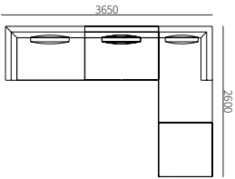
YH26ZH-3 3650*2600*650mm 143.7*102.4*25.6"
