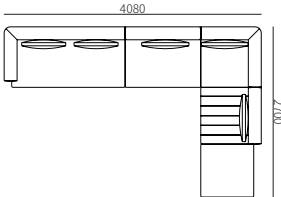
T33ZH-5 4080*2700*700mm 160.6*106.3*27.6"
