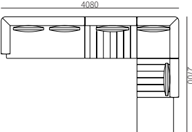
T33ZH-5 4080*2700*700mm 160.6*106.3*27.6"
