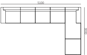
K02ZH-5 5100*3000*760mm 200.8*118.1*29.9"
