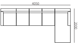
K31ZH-4 4050*2000*760mm 159.4*78.7*29.9"
