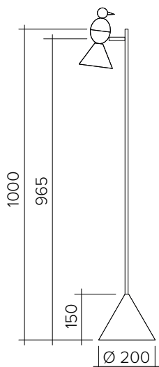
Alouette Floor 1 bird 004OL-F01
