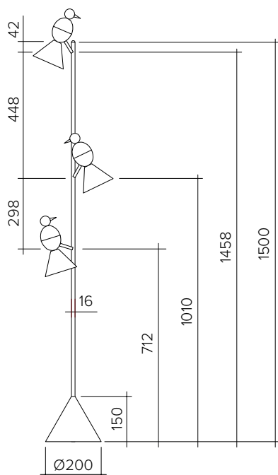
Alouette Floor 3 birds 004OL-F03
