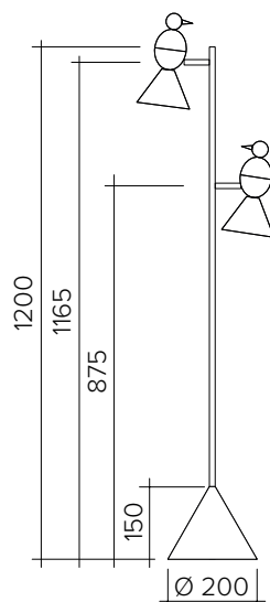
Alouette Floor 2 birds 004OL-F02
