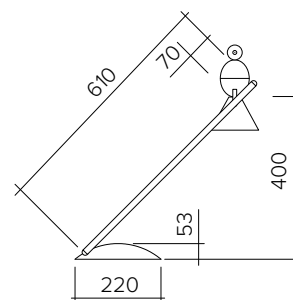
Alouette Desk / slanted 004OL-D02
