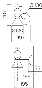
Alouette Wall 004OL-W01
